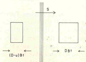
FIG. 5. Geometry for magnetic flux jump condition. Area compression due to shock propagating through magnetic medium at rest is represented. Magnetic field is normal to the page.
